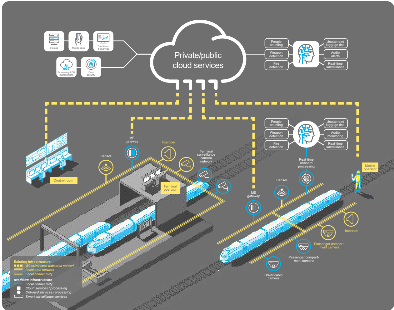
Figure 7: Mission Embedded Solution - system architecture for stationary and onboard surveillance
